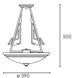
00-5812-B2-98 00-5812-64-98 3 E-27 max. 60W esf. ø45
