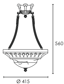
00-2236-S4-55 3 E-27 max. 60W
