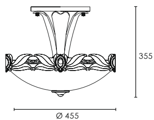
15-2527-G8-55 3 x E-14 esf. ø45 max. 60W
