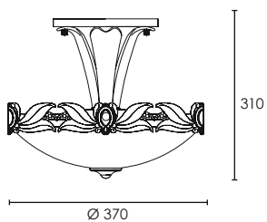
15-2526-G8-55 3 x E-14 esf. ø45 max. 60W
