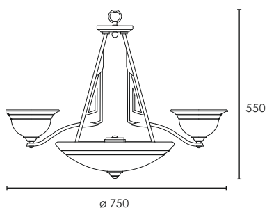
20-5812-B2-98 20-5812-64-98 3 E-27 max. 60W esf. ø45 + 3 E-27 max. 40W esf. ø45
