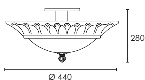
15-2237-S4-55 3 E-14 max. 60W esf. ø45
