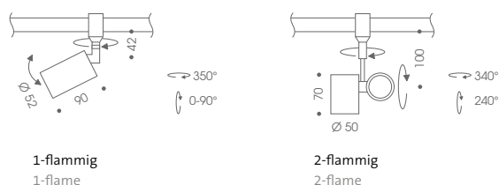
SKIZZE SKETCH
