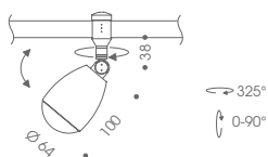
SKIZZE SKETCH
