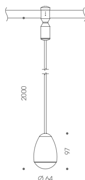
SKIZZE SKETCH
