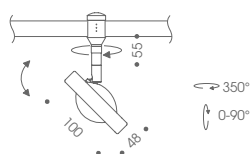
SKIZZE SKETCH
