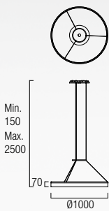
00-3642-BW-M3 (Standard) 00-3646-BW-M3 (Dimmable 1-10V)
