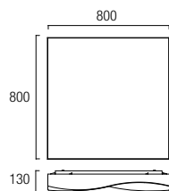
15-5096-S2-M1 (Standard) 15-5120-S2-M1 (Mains dimming)*
