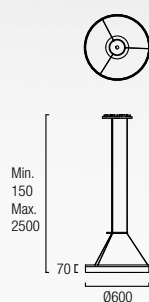
00-0001-BW-M3 (Standard) 00-0641-BW-M3 (Dimmable 1-10V)
