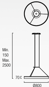
00-0002-BW-M3 (Standard) 00-0642-BW-M3 (Dimmable 1-10V)
